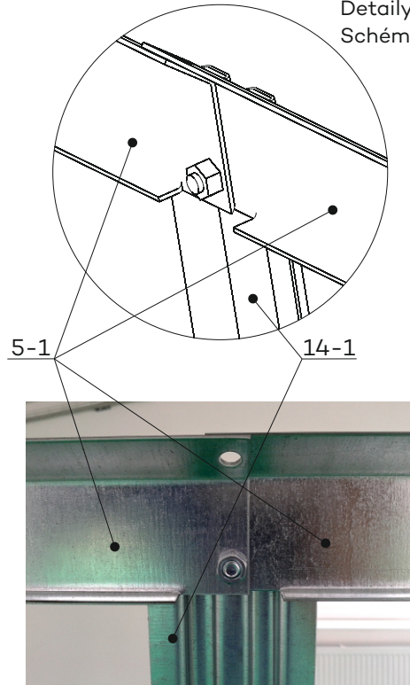
DETAIL G
