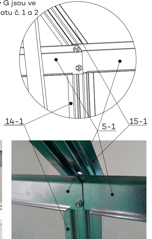
DETAIL G
